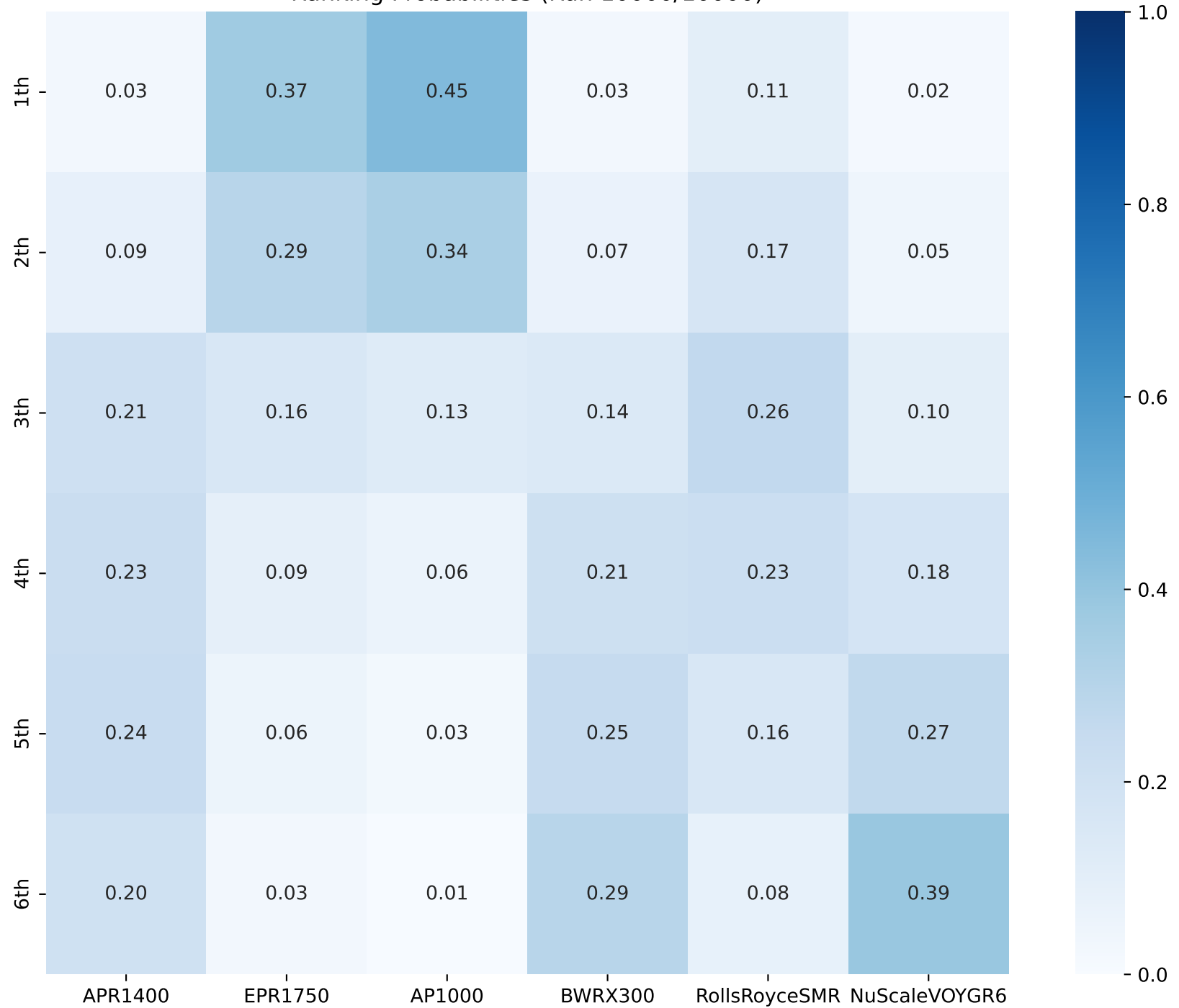
Ranking Probabilities (Run10000/10000)
